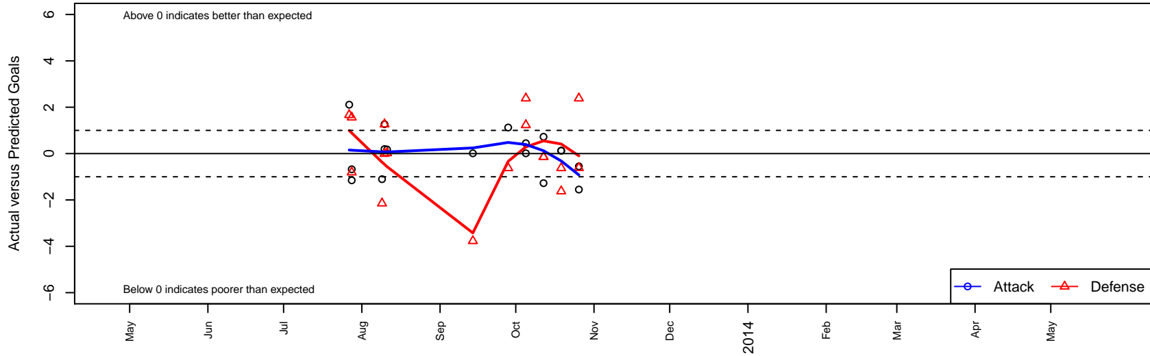
SSC Shadow Elite Blackburn G01 Dots are actual minus expected GF (blue circles) and GA (red triangles). Blue line is smoothed change in attack strength. Red is smoothed change in defense strength.
